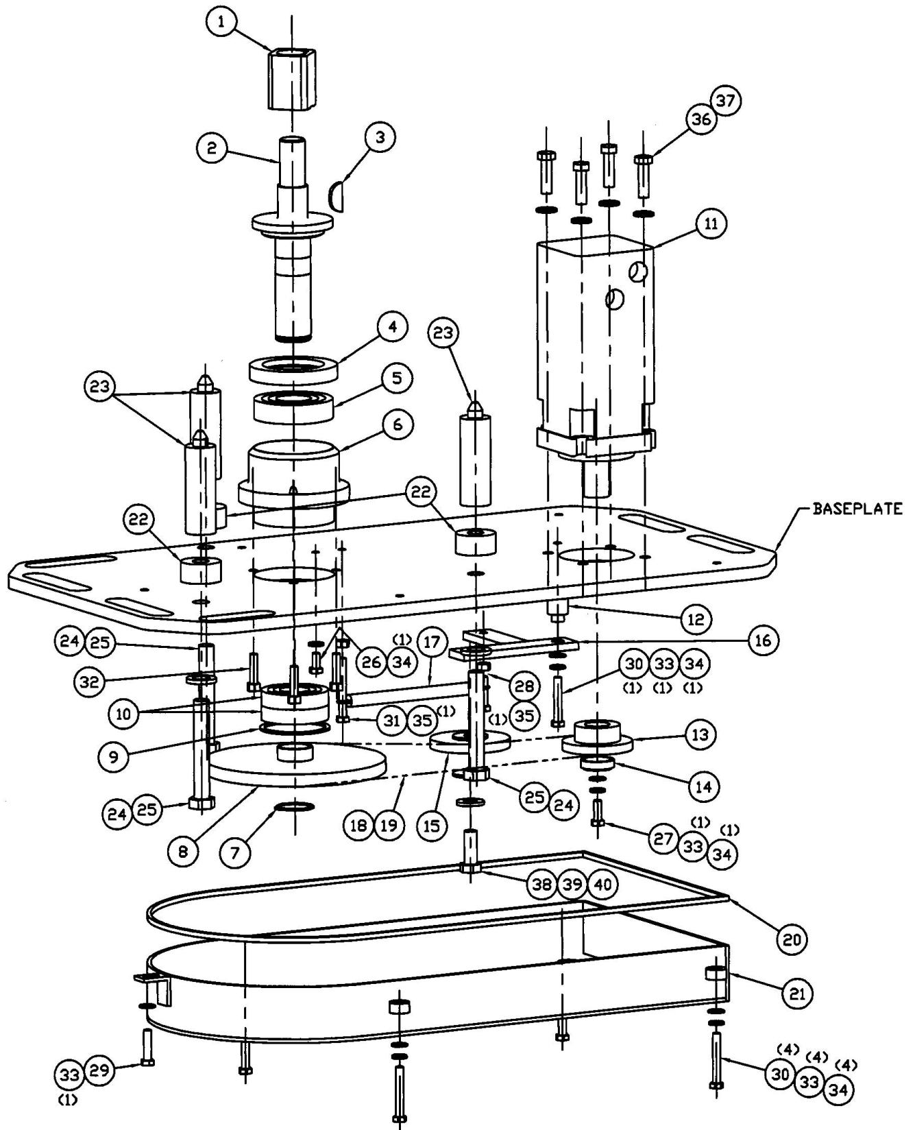
FIGURE 44 POWER TRAIN ASSEMBLY (C-10HHD)
